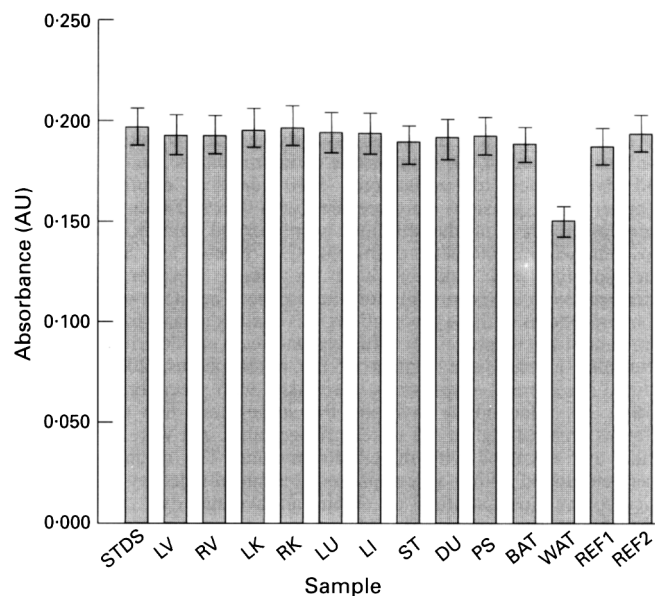
Figure 2 Mean absorbance of dye extracted from blue microspheres isolated from tissues of five rats. Error bars = SD. STDS = recovery standards; LV and RV = left and right ventricles; LK and RK = left and right kidneys; LU = lung; LI = liver; ST = stomach; DU = duodenum; PS = psoas; BAT and WAT = brown and white adipose; REF1 and REF2 = reference blood samples. The mean absorbance of the standards, 0.197 AU, represents 100% recovery.
